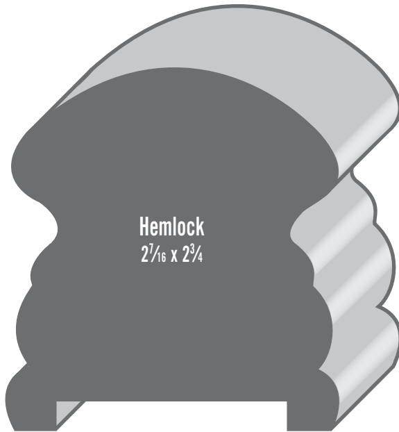
HEMLOCK • FingerJoint H 6019P2 1 5 / 8 Plow (fillet included)
